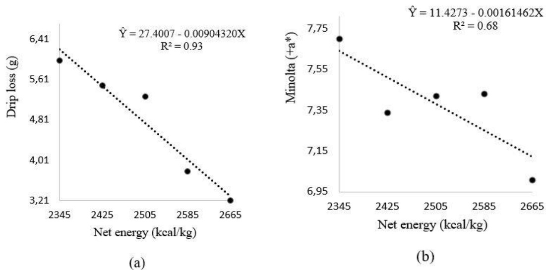
Figure 2 - Graphic representation of drip loss (a) and a* (b) of longissimus dorsi muscle of finishing pigs fed diets with different levels of net energy.
